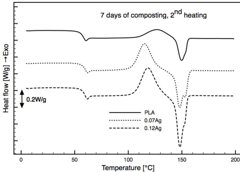
Figure 4: Thermograms of PLA and composites with 0.07 and 0.12 wt% of Ag nanoparticles, after 7 days of composting: second heating scan
