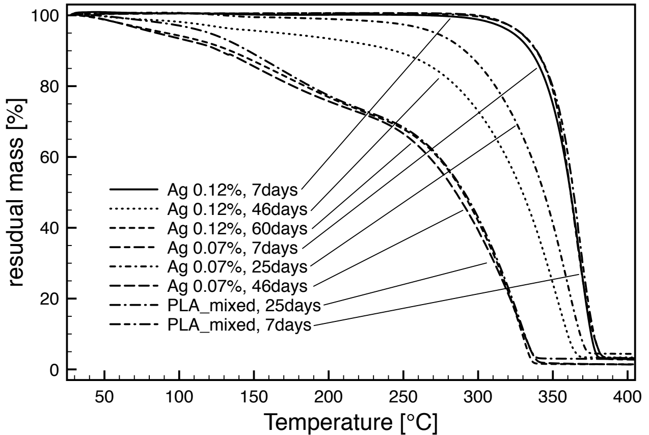
Figure 2: TGA analysis in nitrogen atmosphere for PLA and composites at different biodegradation times
