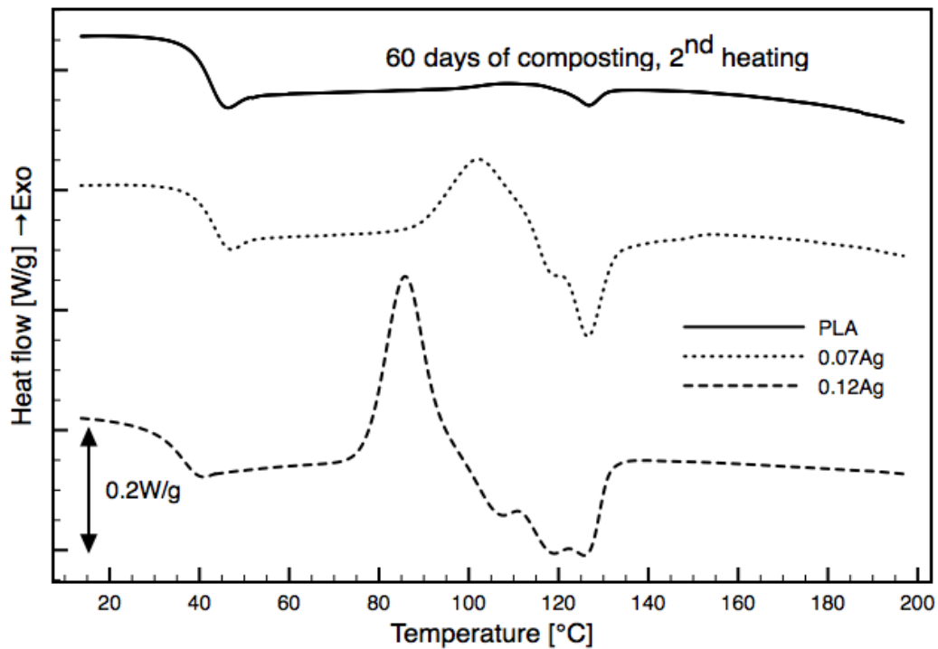
Figure 5: Thermograms of PLA and composites with 0.07 and 0.12 wt% of Ag nanoparticles, after 60 days of composting
