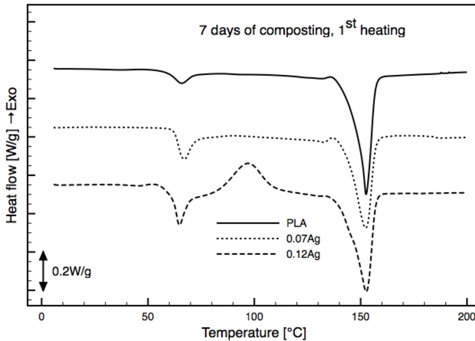
Figure 3: Thermograms of PLA and composites with 0.07 and 0.12 wt% of Ag nanoparticles, after 7 days of composting: first heating scan
